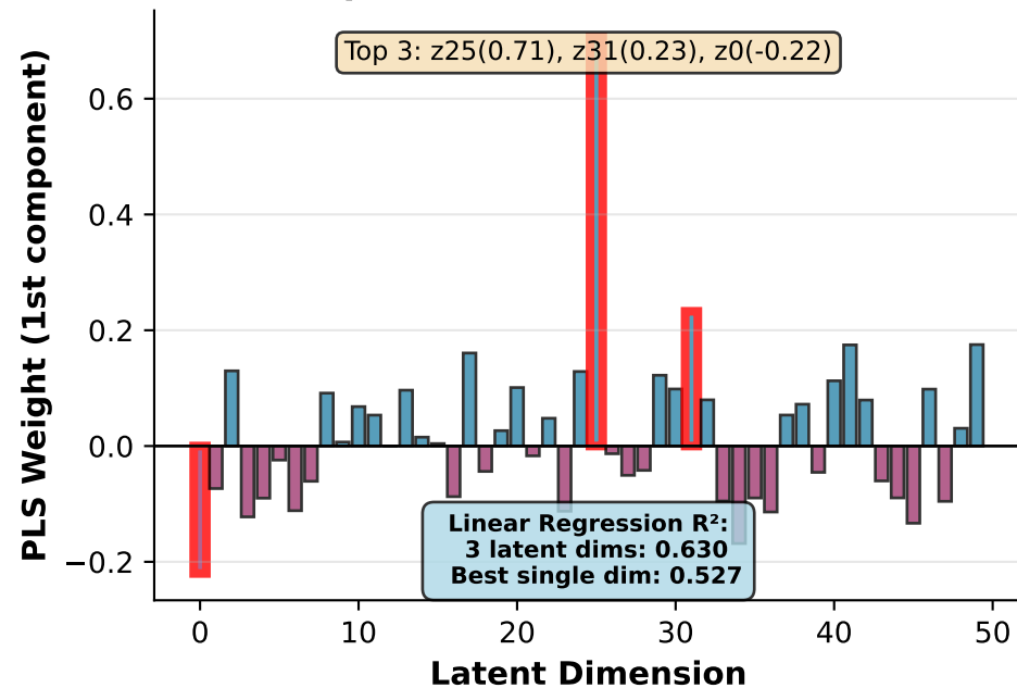
Temporal Variance Optimal Linear Combination
