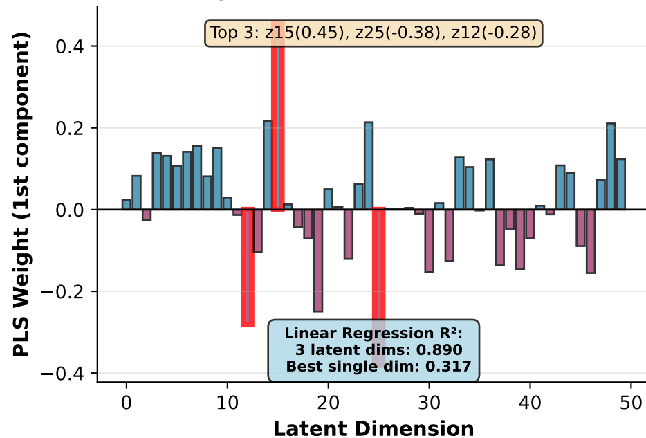
Steady State Optimal Linear Combination
