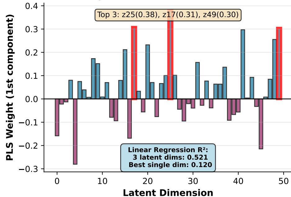
Peak Timing Optimal Linear Combination
